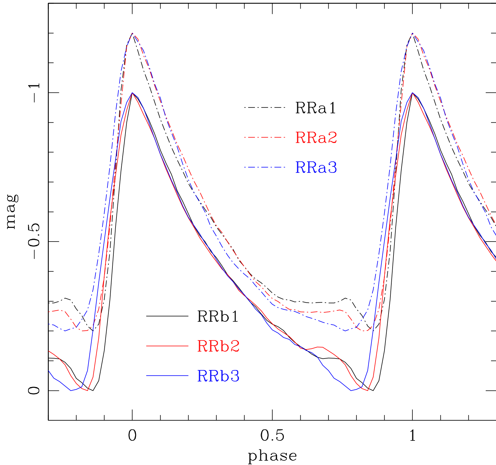
RR Lyrae ab-type Templates in V-band
